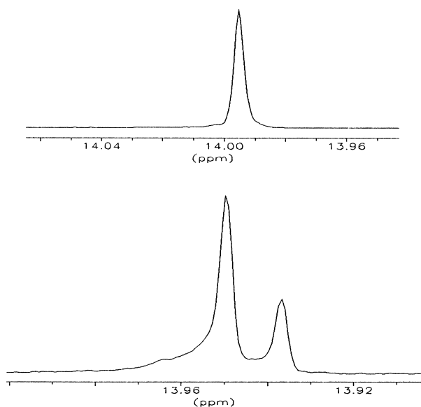
Figure 4. Compound (+)- 2c in toluene- d_8 (top); compound (+)- 2c with TFAE in toluene- d_8 at 223 K showing splitting of the hydroxyl group (bottom).
