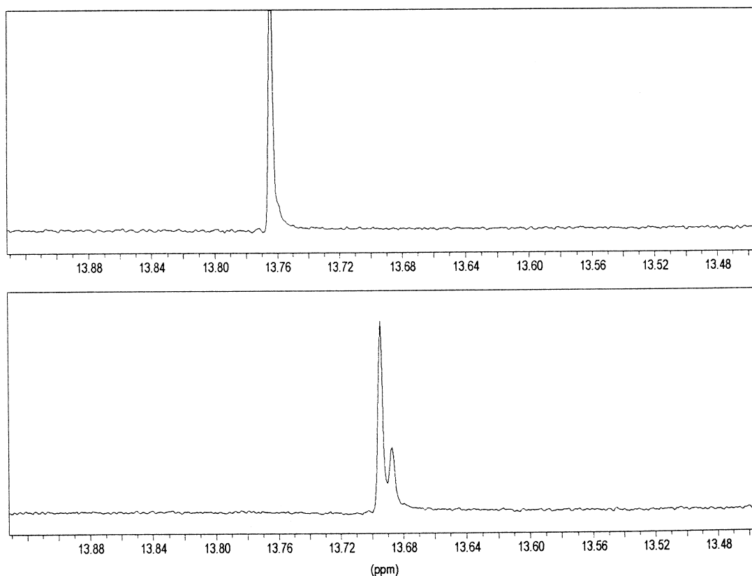
Figure 3. Compound (–)- 2a in toluene- d_8 (top); compound (–)- 2a with TFAE in toluene- d_8 at 223 K showing splitting of the hydroxyl group (bottom).
