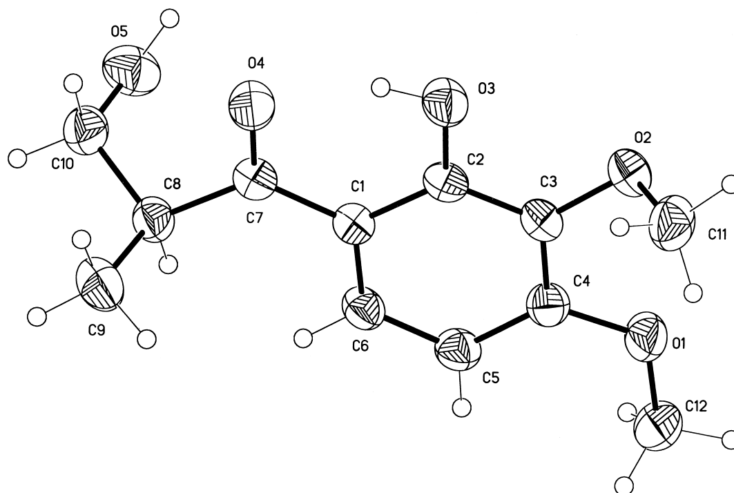
Figure 1. X-ray crystal structure of (±)-3-hydroxy-1-(2-hydroxy-3,4-dimethoxyphenyl)-2-methylpropanone ( 2e ).
