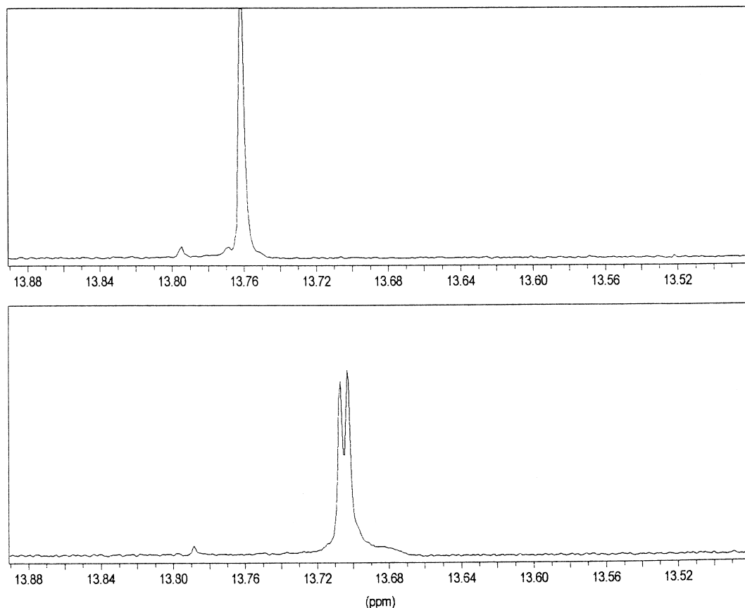
Figure 2. Compound (±)-2a in toluene- d 8 (top); compound (±)-2a with TFAE in toluene- d 8 at 223 K showing splitting of the hydroxyl group (bottom).
